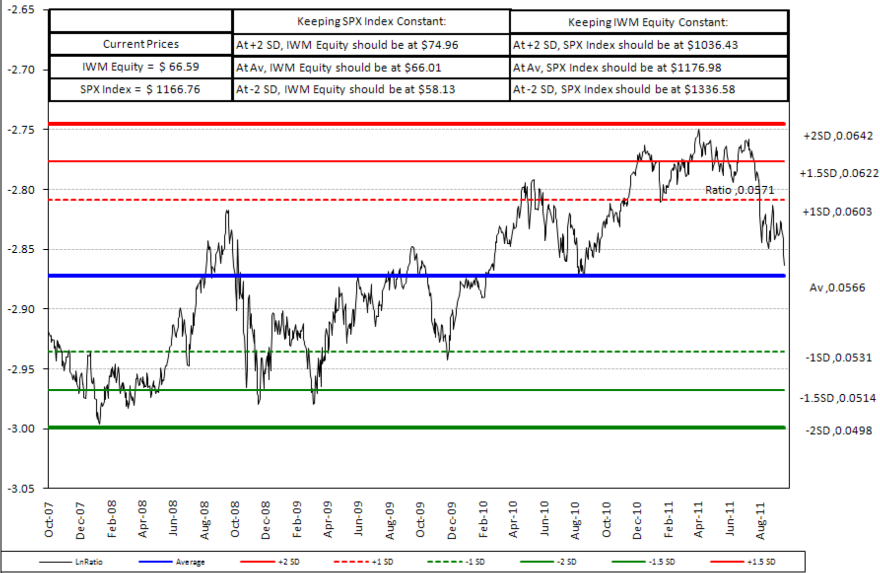
Long IWM Equity and Short SPX Index, Updated till 21 Sep 2011, LAST 4 Years( 1000 TRADING DAYS)
